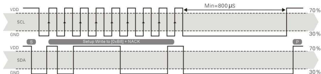
Figure 15: Wake Sensor
