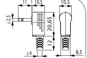
No. MP-022LN (2.5 -2極)
