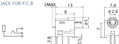
No. MJ-3425M (2.5 -2極)
