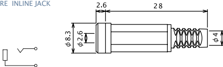
No. MJ-0252S (2.5 -2極)
